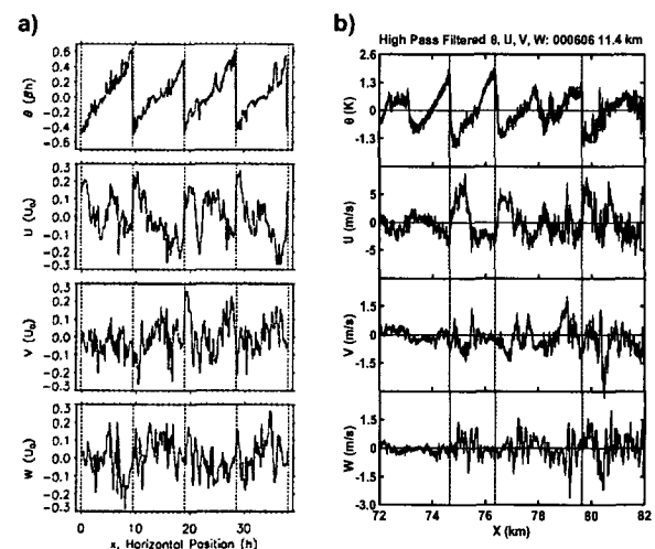
Figure 1. Transects of potential temperature and the u, v, and w wind components for (a) K-H DNS with Ri = 0.2 and non-dimensional time \tau = 77 and (b) aircraft flights over Wales, UK 6 June 2000. For the DNS plots the temperature is scaled by the product of vertical potential temperature gradient and distance from the center of the billow and the winds are scaled by the mean horizontal wind speed.
