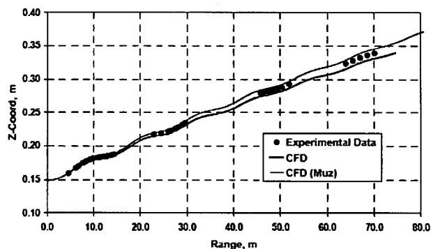
Figure 5. Computed z-distance vs. range
