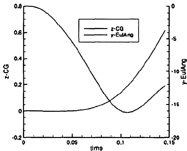
Figure 11. Time history of z -distance (center of gravity) and Euler pitch angle
