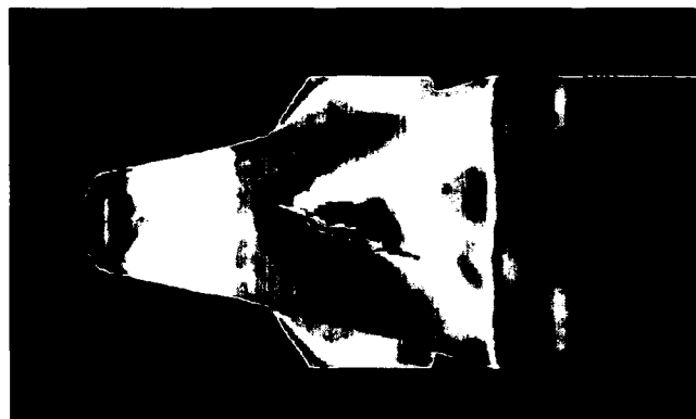
Figure 9. Computed surface pressure contours in the nose section, M = 3.0 , \alpha = 0^\circ
