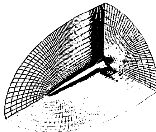
Figure 4. Computational grid
