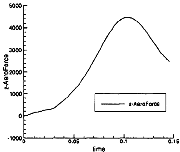
Figure 10. Time history of lift force
