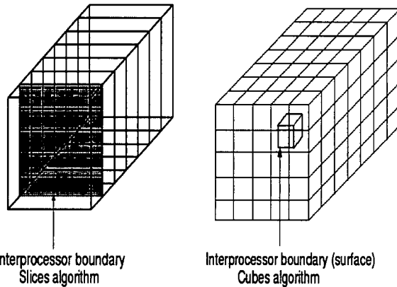
Figure 3. Simple domain decomposition of FDTD domain into "slices" and "cubes." A dedicated processor is assigned to each domain slice or cube and communications are transmitted across interfaces.
