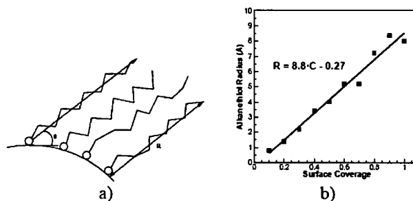
Figure 9. Difference in radial position for the head and tail groups of the alkanethiolate chains at various surface coverage densities, drawing (a) and data (b)
