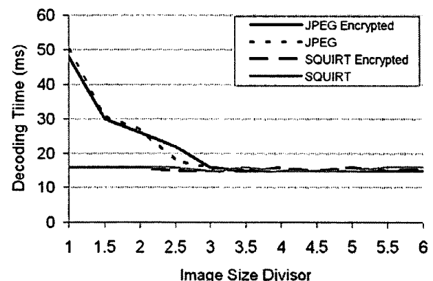
Figure 9. Decoding time vs. image size divisor measurement
