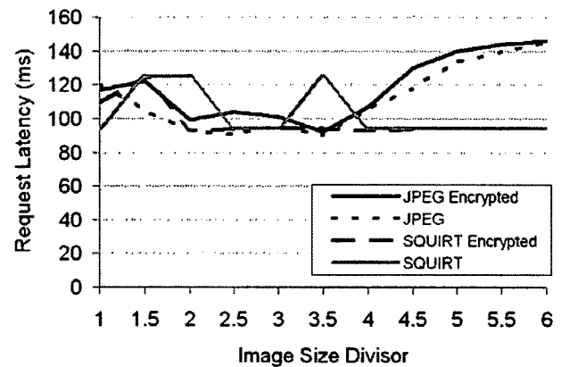
Figure 8. Request latency vs. image size divisor measurement
