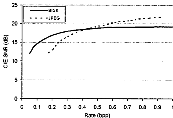
Figure 6. Rate-distortion performance of BISK and JPEG coders
