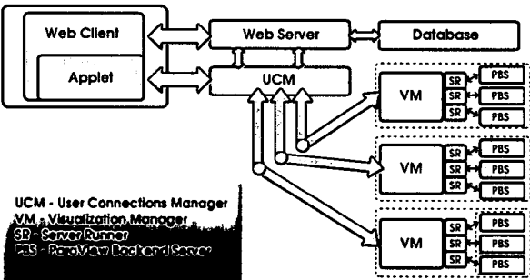
Figure 3. WebVis Architecture
