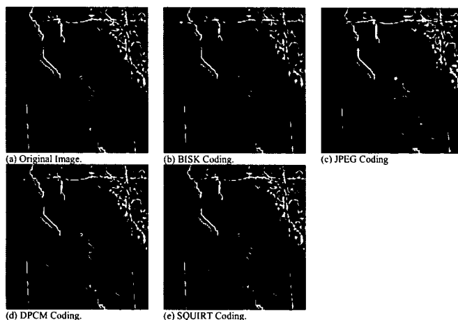
Figure 4. Comparison of original image (a) with images compressed with BISK (b), JPEG (c), DPCM (d), and SQUIRT (e) coders. Unrestricted visualization images courtesy of Derek Irby, Mississippi State University, of Coupled Ocean Atmosphere Mesoscale Prediction System data from Rick Hodur (NRL-MRY). Image analysis performed by James E. Fowler.
