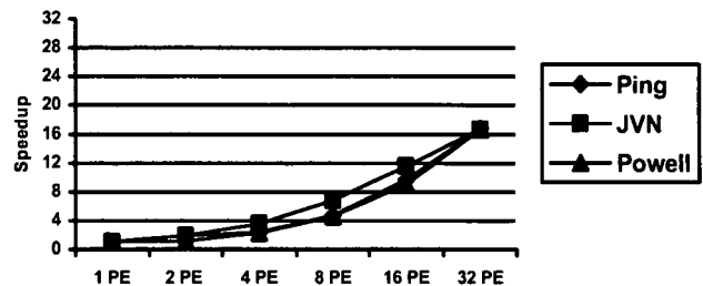
Figure 8. OVERFLOW Scalability
