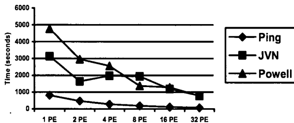
Figure 5. GAMESS Performance
