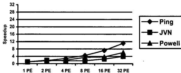
Figure 6. GAMESS Scalability
