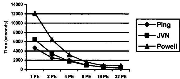
Figure 7. OVERFLOW Performance
