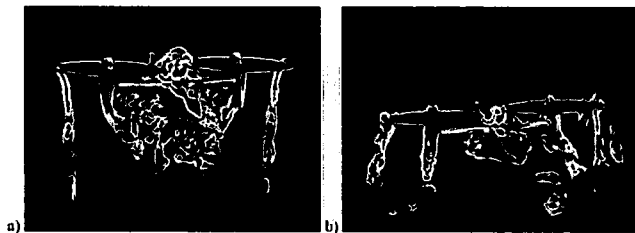
Figure 11. a) Instantaneous cross-plane of vorticity contours for the V-22 in hover and b) Instantaneous cross-plane of vorticity contours for the V-22 in a descent
