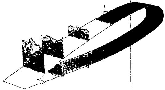
Figure 1. Contours of instantaneous vorticity in four planes along the Aeroespatale-A airfoil at an angle-of-attack of 13.3 degrees and a Reynolds number of 2 \times 10^6
