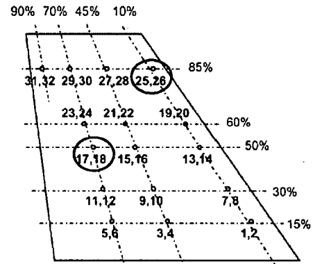
Figure 8. Placement of the F-18 HARV Kulite pressure sensors on the right vertical tail. Odd port numbers are on the inboard section of the tail and even are on the outboard section. Red circles around ports indicates those used in comparing flight test to SADES.
