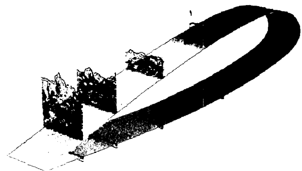
Figure 1. Contours of instantaneous vorticity in four planes along the Aerospatiale-A airfoil at an angle-of-attack of 13.3 degrees and a Reynolds number of 2 \times 10^6
