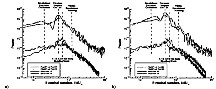
Figure 9. Comparison of Power Spectrum Density from Flight Test and DES Prediction for a) Ports 17 & 18, and b) Ports 25 & 26
