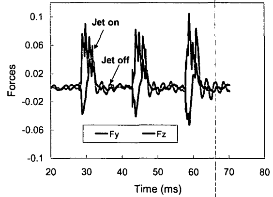
Figure 13. Computed lift and side forces, URANS, M = 0.24 , V_j = 69 \text{ m/s} , \alpha = 0^\circ
