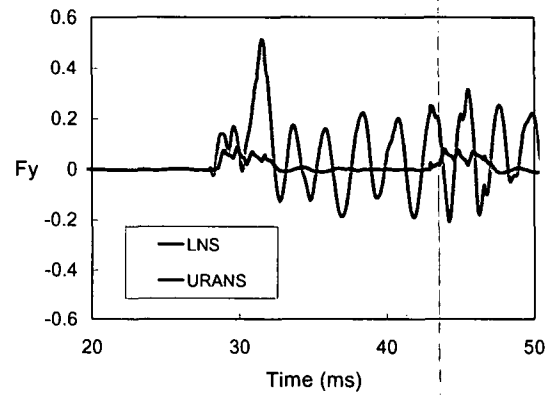
Figure 14. Computed lift forces, URANS and LNS, M = 0.24 , V_j = 69 \text{ m/s} , \alpha = 0^\circ
