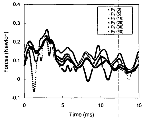
Figure 15. Computed lift force over many spin cycles LNS, V_j = 69 \text{ m/s} , M = 0.24 , \alpha = 0^\circ , Spin = 67 Hz
