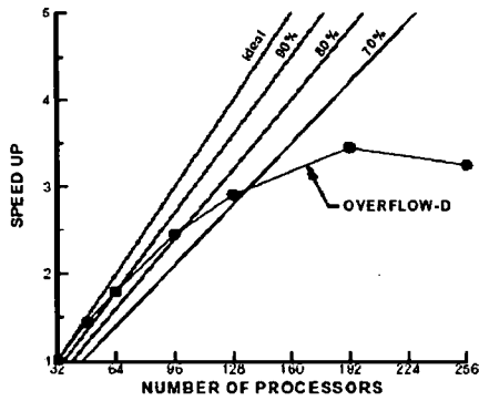
Figure 4. OVERFLOW-D parallel scalability
