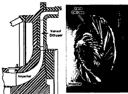
Figure 2. High-speed centrifugal compressor, CC3, validation case
