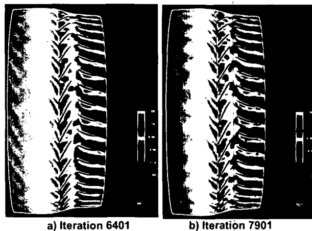
Figure 7. Axial velocity contours near the casing during stall inception at iteration 6401 and 7901, full-annulus simulation
