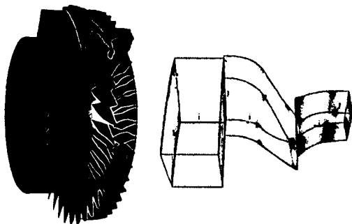
Figure 4. Three-blade-row Grid Model for the Stage 35 simulation
