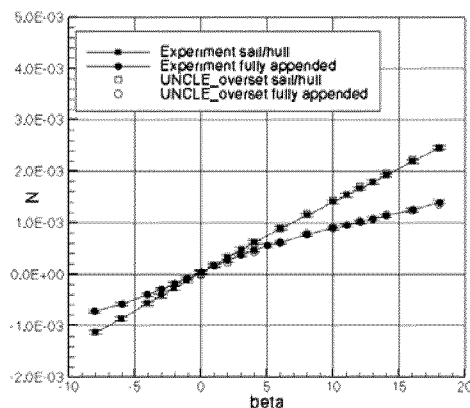
Figure 19: Comparison of yaw moment coefficient.
