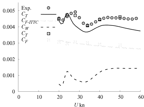
Figure 8: Resistance coefficients at model scale, Configuration 6. (○) experiment; (---) thin-ship theory with no form factor; (□) FLUENT
