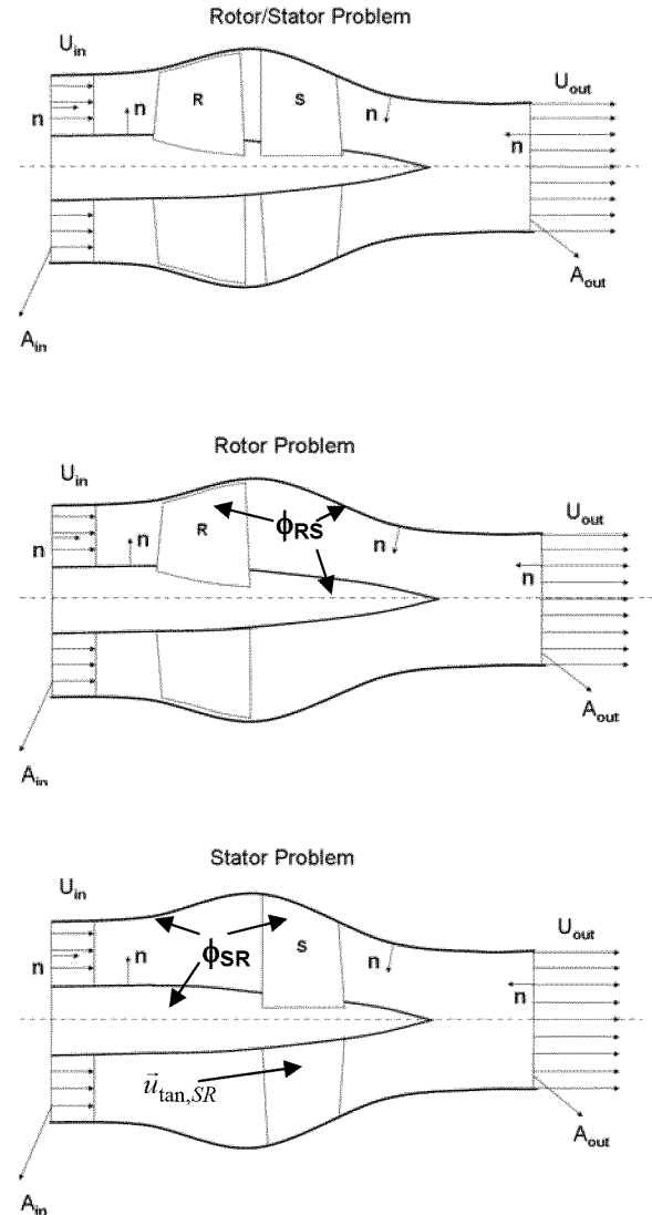
Figure 2: Schematic showing: (a) the combined rotor/stator problem, (b) the rotor problem, and (c) the stator problem. Problems (b) and (c) are solved in sequence with the (time-averaged) effects of one on the other being accounted for in an iterative sense.
