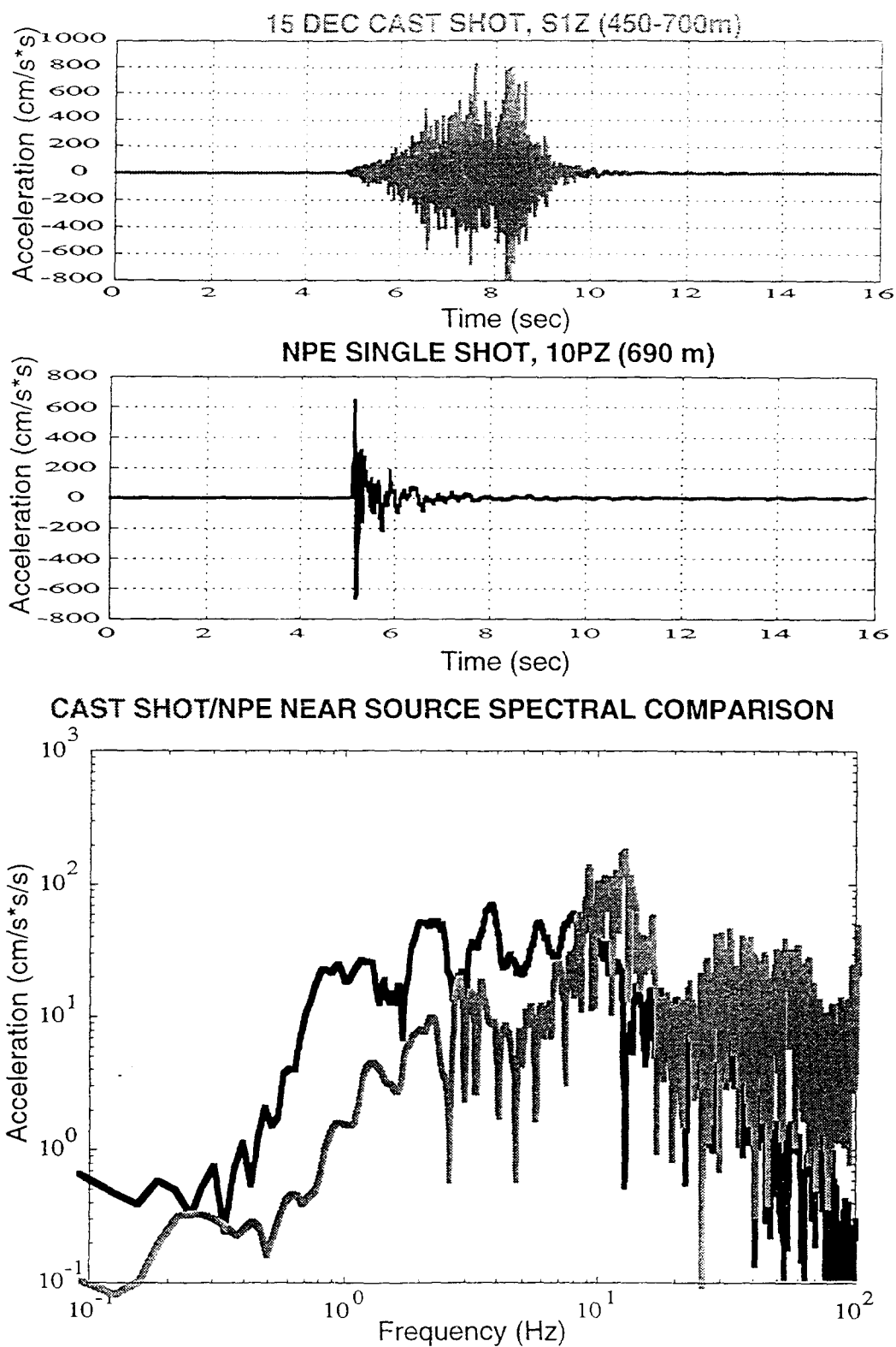
Figure 5: Comparison of near-source accelerations from a Cast Blast (top) and the NPE (bottom).
